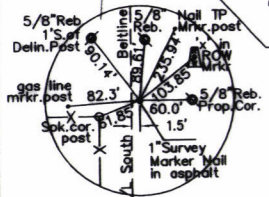
Southwest Corner Section 15, T22N, R55W Found 1" Survey Marker Nail in Asphalt
