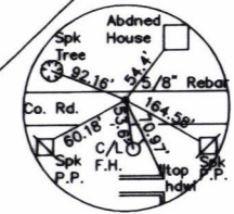
SOUTH QUARTER CORNER Section 15, T22N, R55W Found 5/8" Rebar
